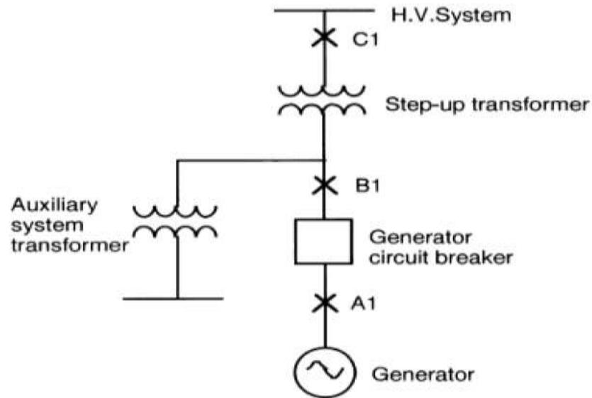
Fig.3.4 Single-line diagram of unit generator system
