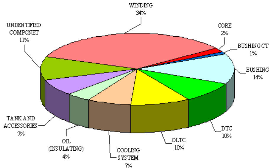
Fig. 3 Number of transformer stoppages versus components
