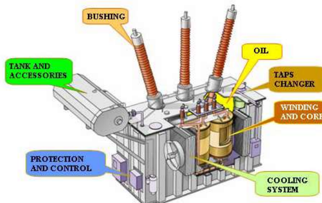
Fig.2 Power Transformers
