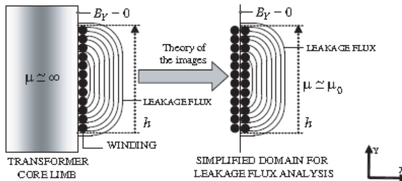
Fig.1 The leakage flux in three-phase transformers
