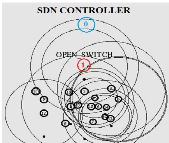
Figure 5 SDN Network Packet Drop
