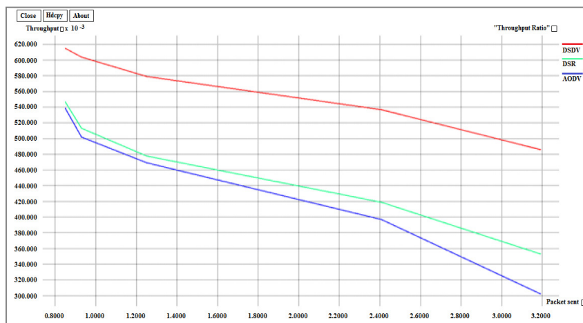
Figure 6 Packet Sent Vs Throughput
