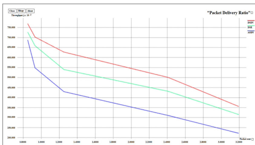
Figure 8 Packet Sent Vs Packet Delivery Ratio
