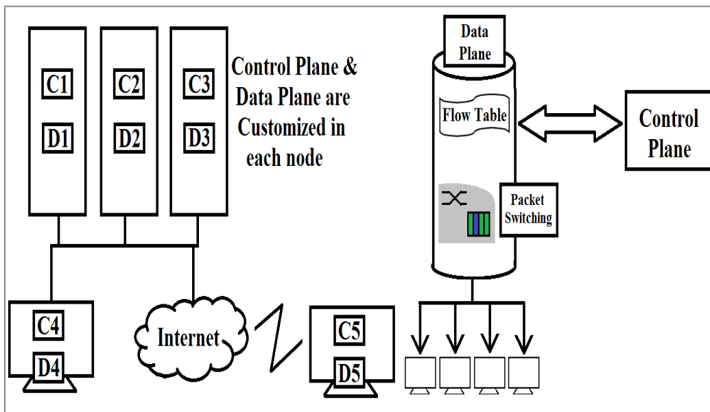
Figure 1 Traditional Network Vs Software Defined Network
