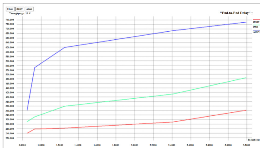
Figure 7 Packet Sent Vs End-to-End Delay
